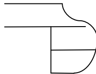
2-1/4" Ogee Bullnose
