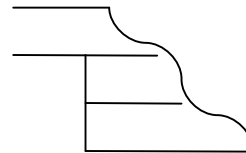
2-1/4" Double Ogee
